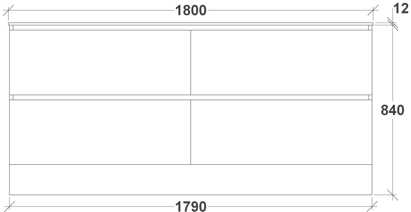
FRONT VIEW
