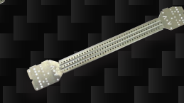
TELESCOPIC NOG BRACKETS Telescopic galvanized steel bracket supports brass wing backs and Polymer Lugged Elbows (BLE's). Ideal for timber or steel frame projects. BK3 - 260mm to 400mm BK4 - 355mm to 610mm
