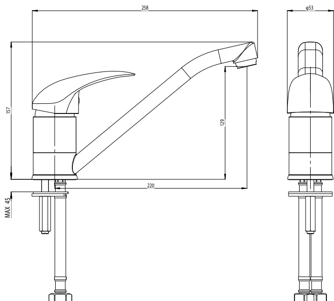
Posh Bristol MK2 Sink Mixer
