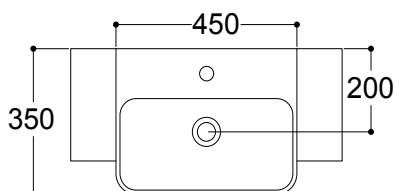
Sheer Semi Recessed Basin 450mm
