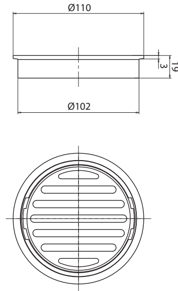
Mizu Drift Brass Trapscrew Grate Round 100mm
