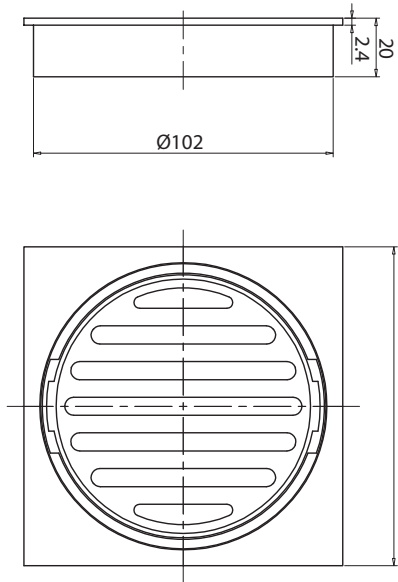
Mizu Drift Brass Trapscrew Grate Square 100mm
