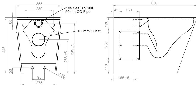
MODEL PCAMP Side and Rear Elevation
