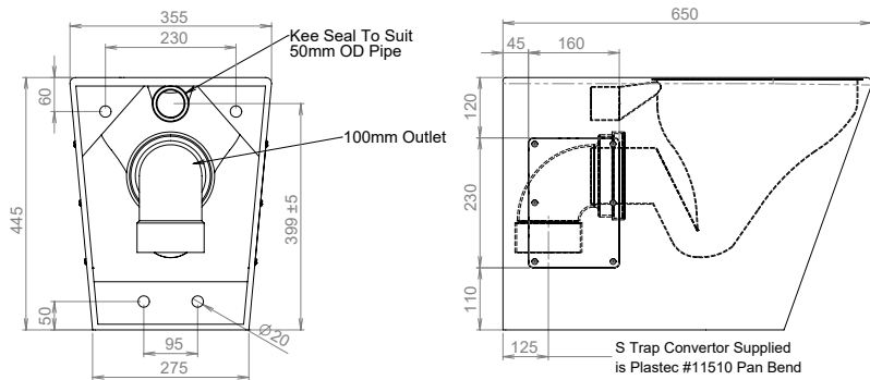
MODEL PCAMS Side and Rear Elevation
