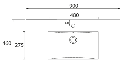
900mm Vanity Top - Centre Bowl - 1 Taphole - Top View
