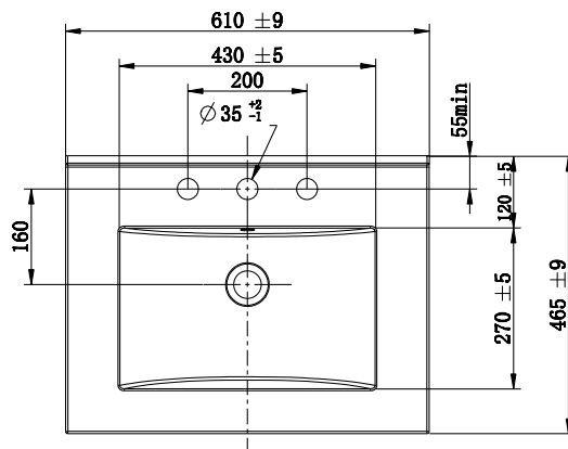
600mm Vanity Top - 3 Taphole - Top View
