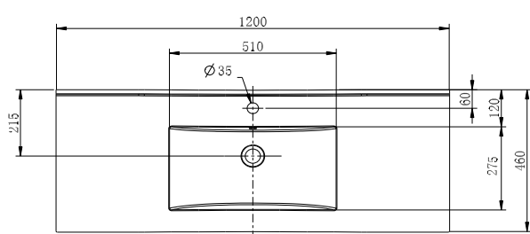
1200mm Vanity Top - Centre Bowl - 1 Taphole - Top View
