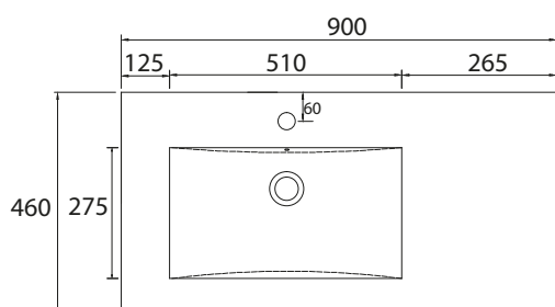
900mm Vanity Top - Left Hand Bowl - 1 Taphole - Top View
