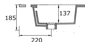
900mm Vanity Top - Side View
