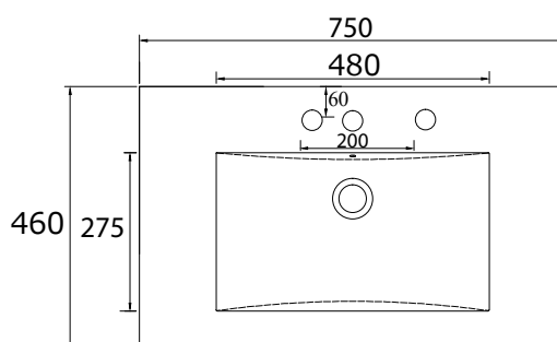
750mm Vanity Top - Centre Bowl - 3 Taphole - Top View
