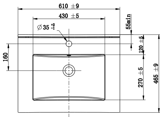
600mm Vanity Top - 1 Taphole - Top View
