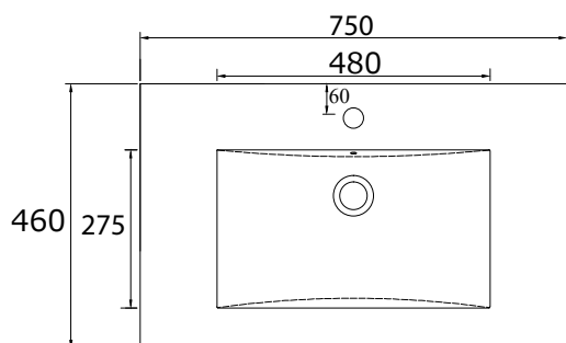
750mm Vanity Top - Centre Bowl - 1 Taphole - Top View
