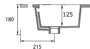
750mm Vanity Top - Side View
