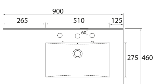
900mm Vanity Top - Right Hand Bowl - 3 Taphole - Top View
