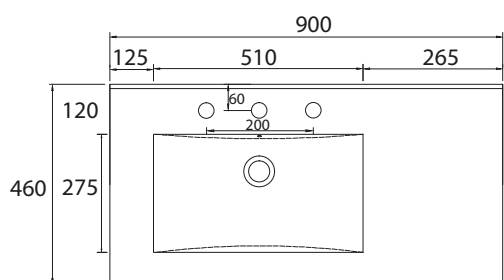
900mm Vanity Top - Left Hand Bowl - 3 Taphole - Top View
