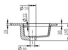
1200mm Vanity Top - Side View
