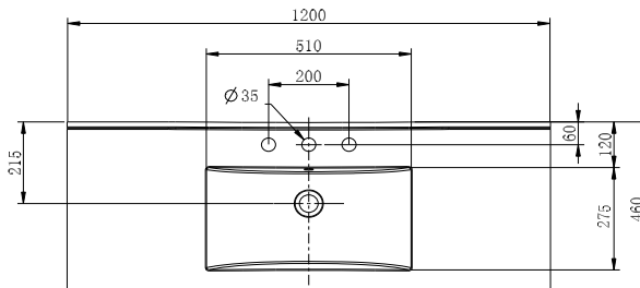
1200mm Vanity Top - Centre Bowl - 3 Taphole - Top View
