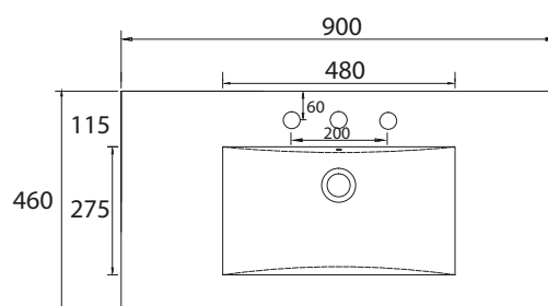
900mm Vanity Top - Centre Bowl - 3 Taphole - Top View
