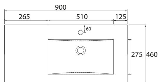
900mm Vanity Top - Right Hand Bowl - 1 Taphole - Top View
