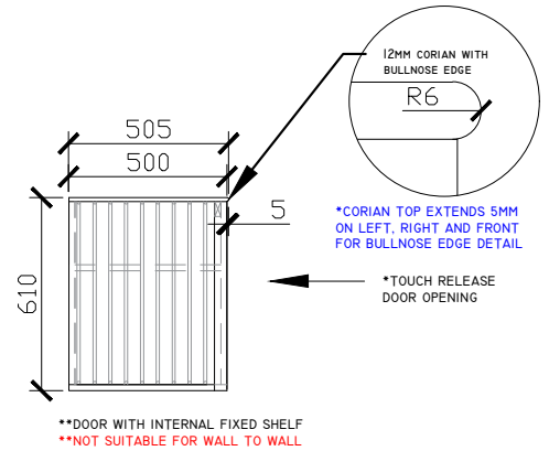
SIDE VIEW for all sizes
