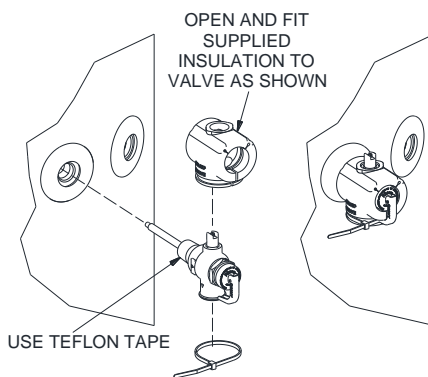
preformed insulation collar
