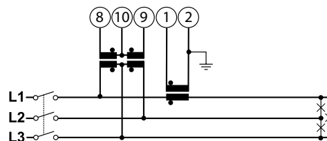
Connection from 1 TA and 2TV
