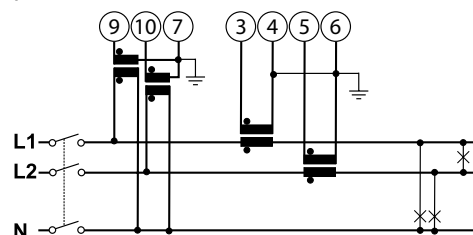
Connection from 2 CT and 2 VT/PT
