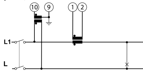
Connection from 1 TA and 1 TV
