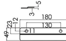
Floor Clip
