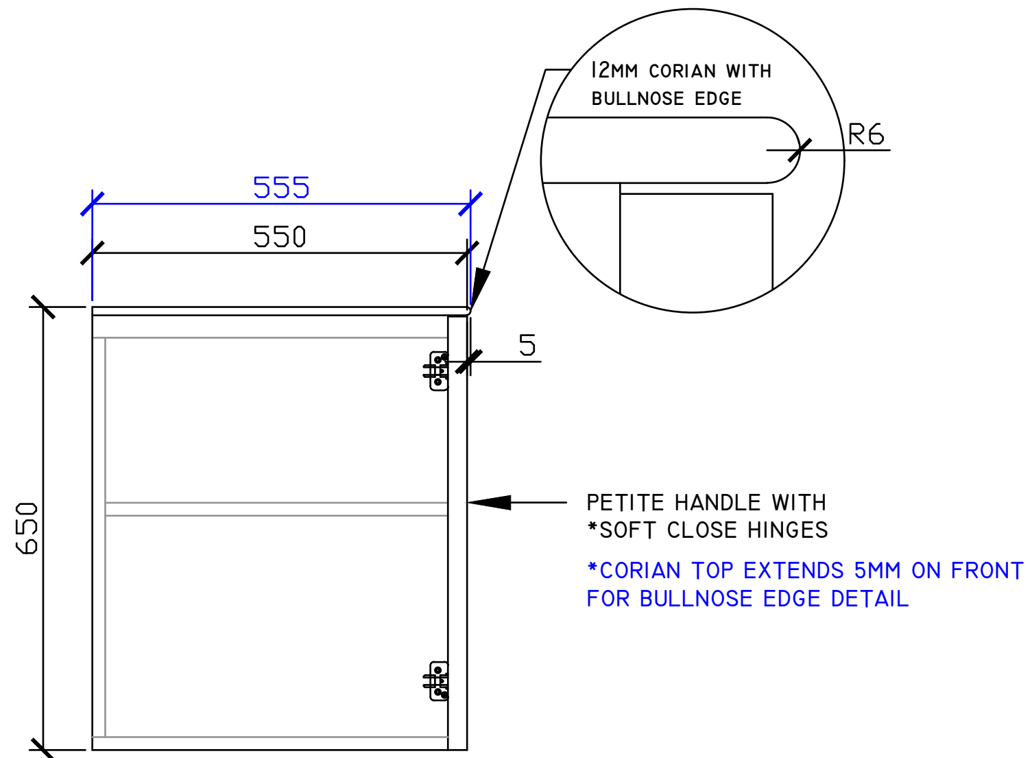
**DOOR WITH INTERNAL FIXED SHELF
