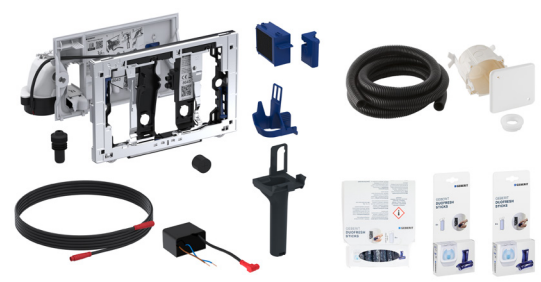
1804981 Geberit DuoFresh Odour Extraction System
