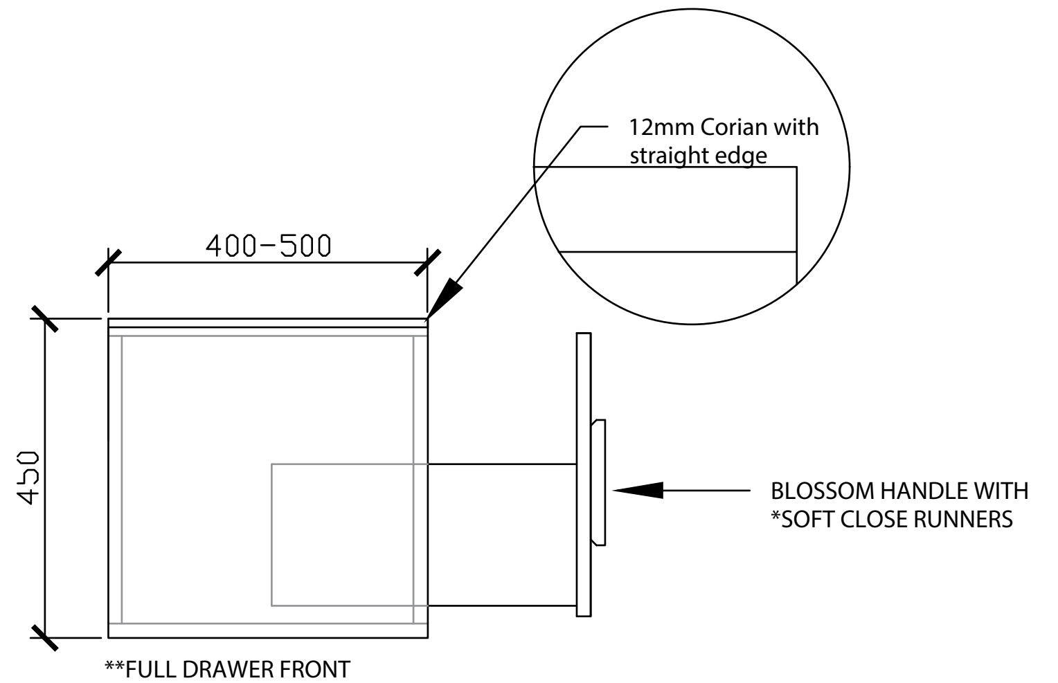
SIDE VIEW for 500 & 600
