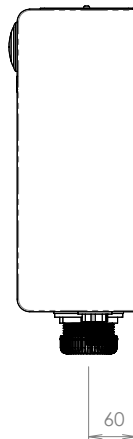
MODEL FCS Side Elevation
