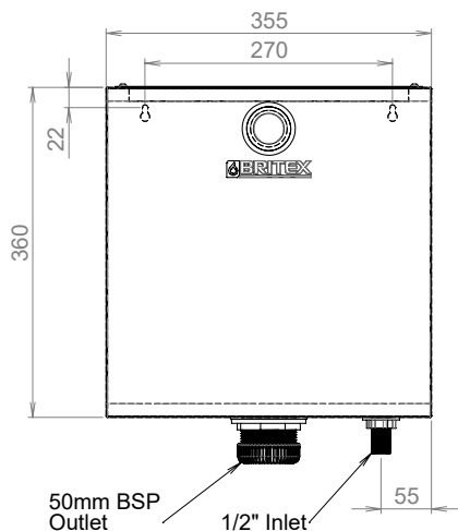
MODEL FCS Front Elevation
