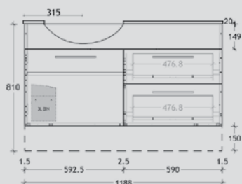
Essence MK II Semi-Recessed 1200mm Offset Wall Hung: MER1200WHD With Kick: MER1200WKD
