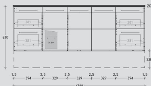
Essence MK II 1800mm Single Bowl: With Kick: ME1800WKS
