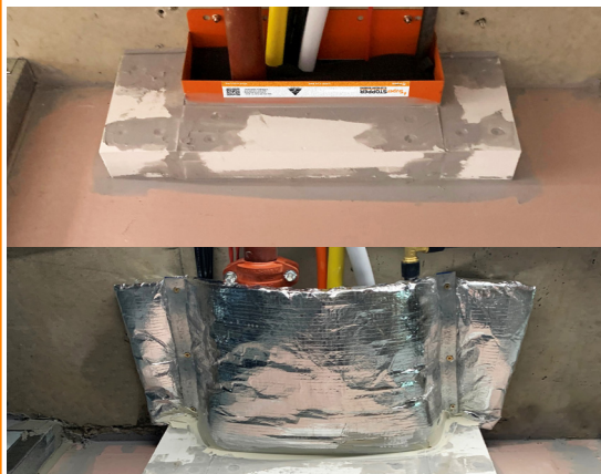
The SuperSTOPPER® can be installed offset to the wall using strips of FyreBOARD Maxilite® to locally thicken the penetration.
