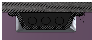
TWrap secured through flat steel section 30x1x300mm
