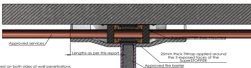
DETAIL P
