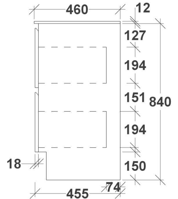
SIDE VIEW
