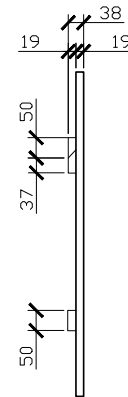
SIDE VIEW for all sizes
