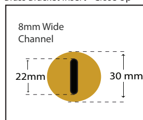
Brass Bracket Insert - Close Up
