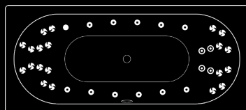
PROFESSIONAL SYSTEM 36 JETS (for double-ended baths) To suit models: 663, 664, 665
