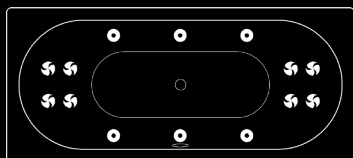
14 JETS (for double-ended baths) To suit models: 663, 664, 665
