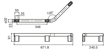
Drift 135° Angled Grab Rail Left Hand
