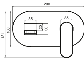
Soothe Wall Basin Mixer Set
