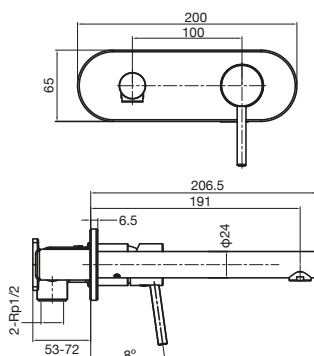
Drift MK2 Wall Bath Mixer Tap Set
