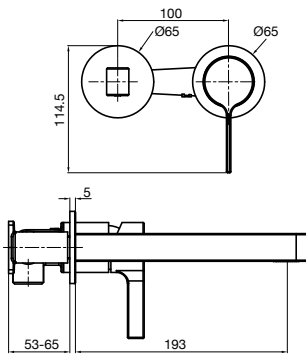
Stream Wall Basin Mixer Set with 2 Cover Plate Design
