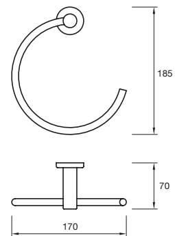
Drift Towel Ring
