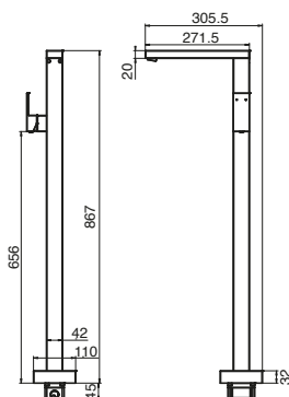
Bloc Floor Bath Mixer
