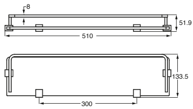
Bloc Glass Shelf with Railing
