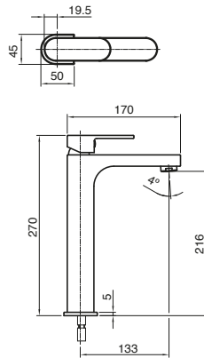
Soothe Extended Basin Mixer
