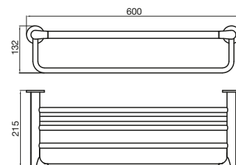
Silk Towel Rack
