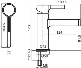
Stream Basin Mixer
