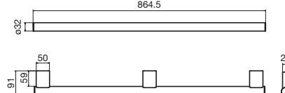
Drift Straight Grab Rail 860mm
