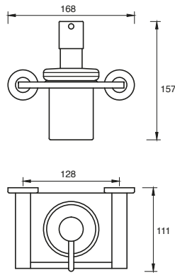
Drift Wall Mounted Soap Dispenser
