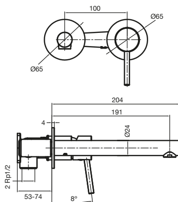
Drift MK2 Wall Basin Mixer Set with 2 Cover Plate
