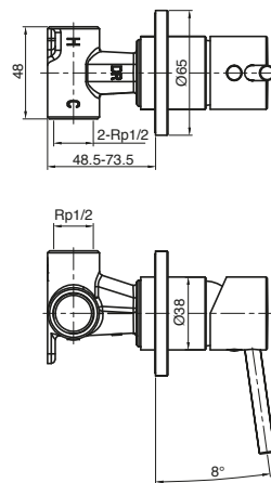
Drift MK2 Shower Mixer
