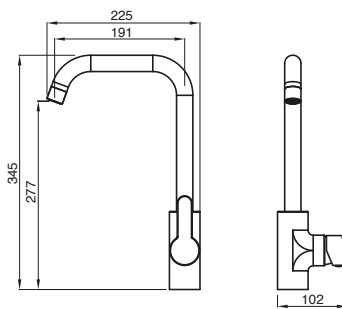
Soothe Square Gooseneck Sink Mixer
