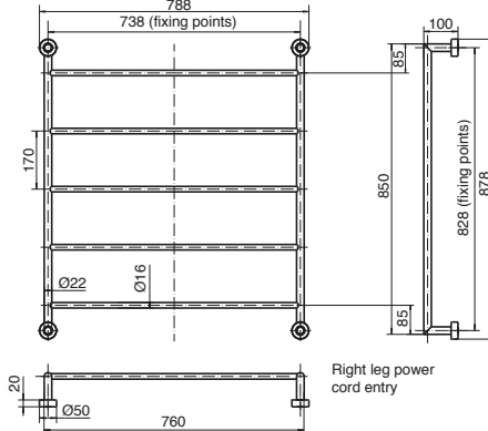
Drift Heated Towel Rail 760 x 850
