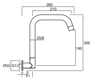
Drift Gooseneck Wall Bath Outlet
