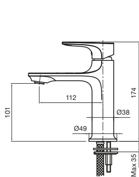
Silk Basin Mixer
