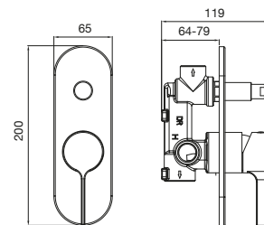
Stream Shower Mixer with Diverter
