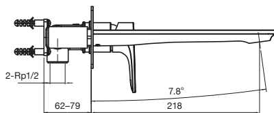
Silk Wall Bath Mixer Set
