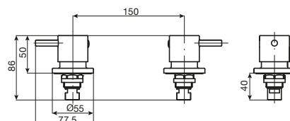
Drift Wall Top Assembly
