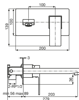
Bloc Wall Basin Mixer Set
