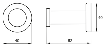
Drift Robe Hook
