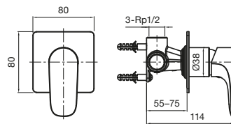
Silk Shower Mixer
