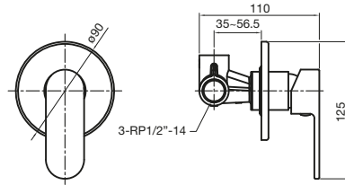
Soothe Shower Mixer
