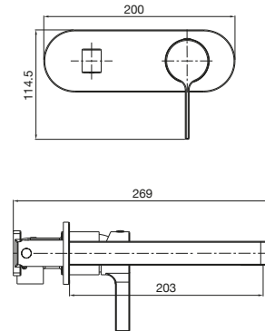
Stream Wall Basin Mixer Set
