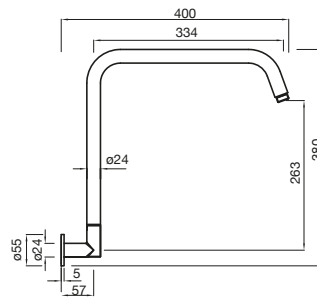
Drift Gooseneck Shower Arm
