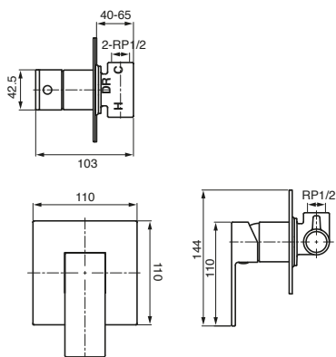
Bloc Shower Mixer
