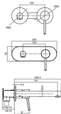
Drift MK2 Wall Basin Mixer Set
