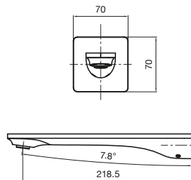
Silk Bath Outlet
