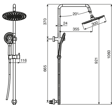
Drift Twin Waterrail Shower
