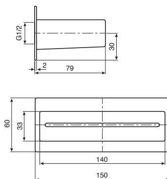
Bloc Waterfall Bath Outlet
