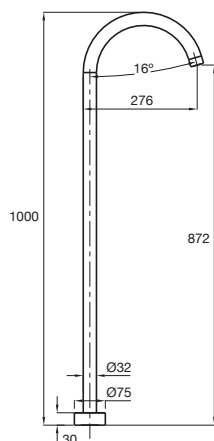
Drift MK2 Floor Bath Outlet
