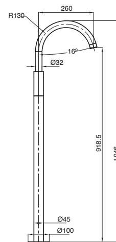
Drift MK2 Shower Mixer with Diverter
