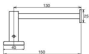
Drift Straight Toilet Roll Holder
