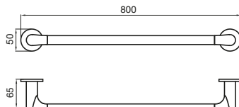
Silk Single Towel Rail
