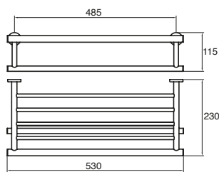
Drift Towel Rack
