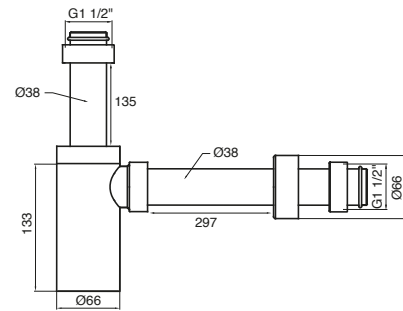
Drift Bottle Trap 40mm
