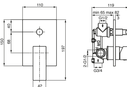
Bloc Shower Mixer with Diverter
