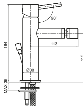
Drift MK2 Bidet Mixer
