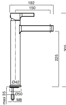
Stream Extended Basin Mixer
