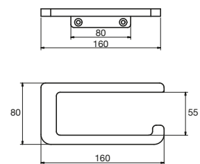
Soothe Curved Toilet Roll Holder
