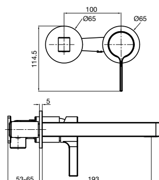
Drift Mk2 Wall Bath Mixer Set with 2 Cover Plate
