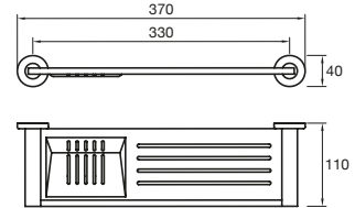
Drift Metal Shelf and Soap Dish
