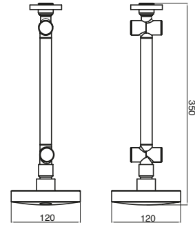
Drift Hi-Rise Shower
