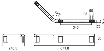
Drift 135° Angled Grab Rail Right Hand
