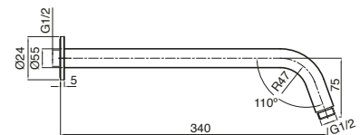
Drift Wall Straight Shower Arm
