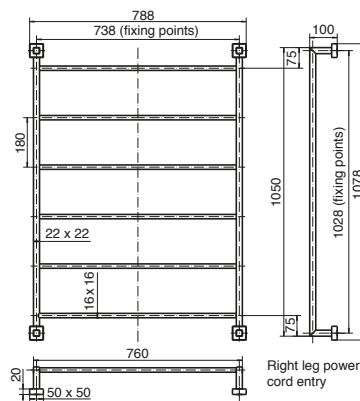
Bloc Heated Towel Rail 760 x 1050
