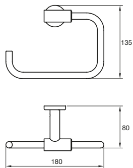
Drift Square Guest Towel Holder
