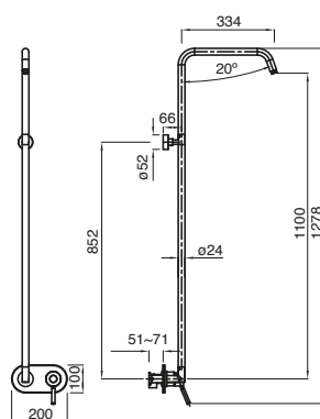
Drift Column Shower with Mixer
