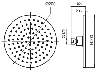
Drift Overhead Shower 200mm
