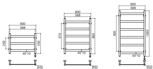
Stream Heated Towel Rail
