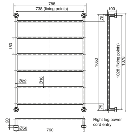
Drift Heated Towel Rail 760 x 1050
