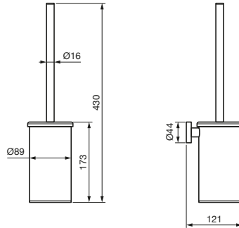
Silk Toilet Brush Holder Metal
