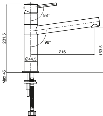
Drift MK2 Sink Mixer
