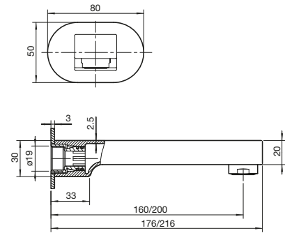
Soothe Basin Outlet
