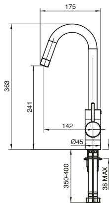
Drift MK2 Gooseneck Sink Mixer
