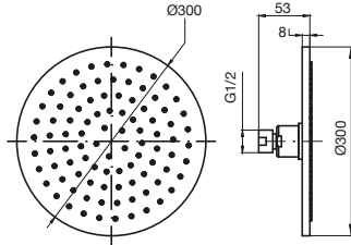
Drift Overhead Shower 300mm
