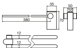
Soothe Swivel Double Towel Bar
