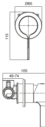
Stream Shower Mixer
