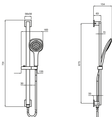
Bloc Single Watterail Shower
