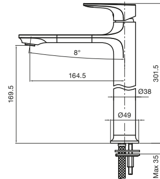
Silk Extended Basin Mixer
