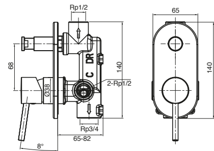
Drift MK2 Shower Mixer with Diverter
