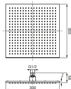
Bloc Overhead Shower
