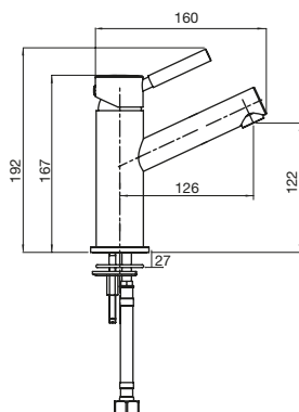
Drift Basin Mixer
