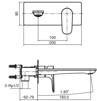
Silk Wall Basin Mixer Set
