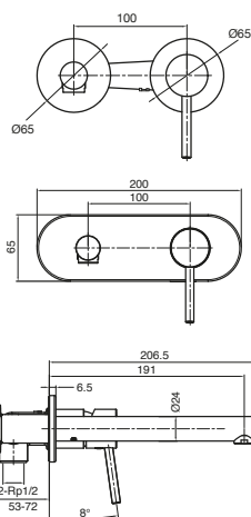
Drift MK2 Wall Basin Mixer Set
