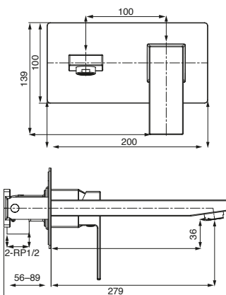
Bloc Wall Basin Set
