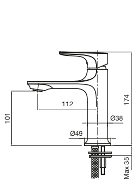
Silk Basin Mixer
