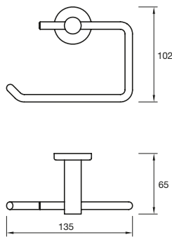
Drift Loop Toilet Roll Holder
