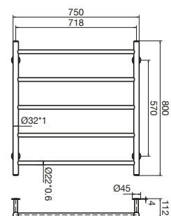
Drift MK2 Low Voltage Heated Towel Rail 750 x 800
