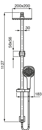
Bloc Twin Witerrail Shower
