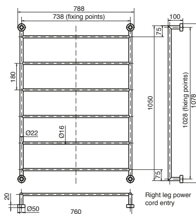
Drift Heated Towel Rail 760 x 1050
