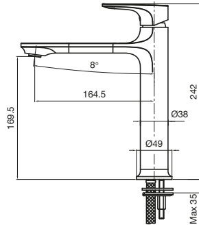
Silk Medium Basin Mixer
