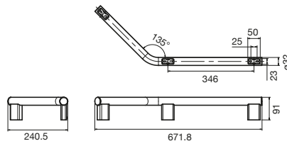
Drift 135° Angled Grab Rail Right Hand
