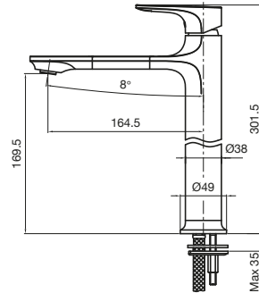
Silk Extended Basin Mixer
