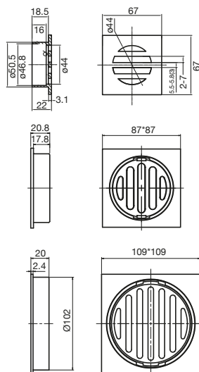
Drift Trapscrew Grate Square and Round 50 / 80 / 100mm
