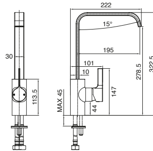
Stream Sink Mixer
