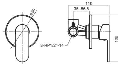
Soothe Shower Mixer
