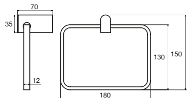
Soothe Towel Ring
