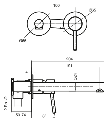
Drift MK2 Wall Basin Mixer Set with 2 Cover Plate
