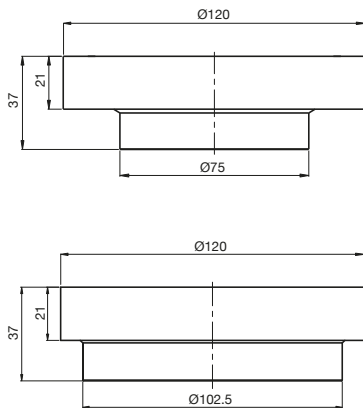
Drift Tile Insert Waste 80 / 100mm
