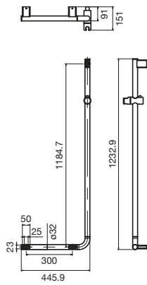
Drift 90 ° Angled Shower Grab Rail
