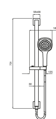
Bloc Single Witerrail Shower
