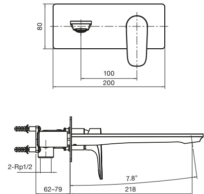
Silk Wall Bath Mixer Set
