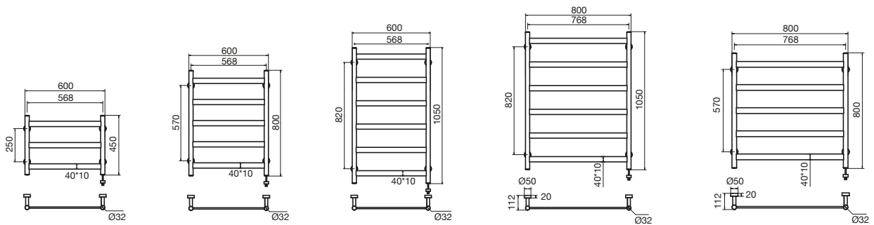
Stream Heated Towel Rail
