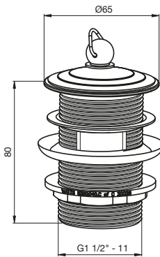
Drift Plug and Waste with Overflow
