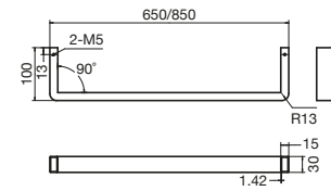
Stream Single Heated Towel Rail
