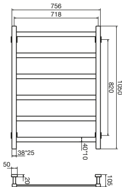
Bloc MK2 Low Voltage Heated Towel Rail 750 x 1050
