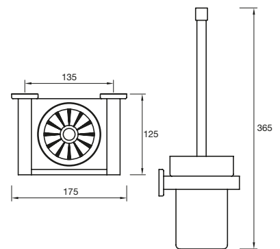
Drift Toilet Brush and Holder
