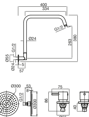
Drift Gooseneck Shower Set
