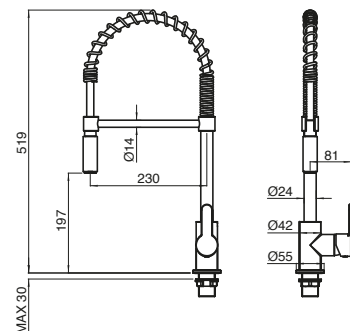
Soothe Pulldown Sink Mixer
