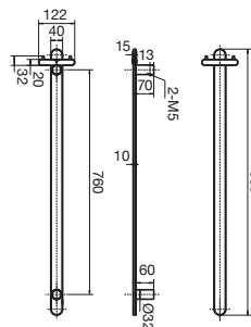
Soothe Vertical Heated Towel Rail
