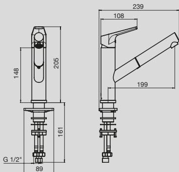
Solus MK3 Pull Out Sink Mixer
