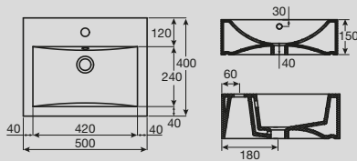
Solus Counter Basin
