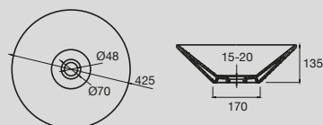
Solus Vessel Basin 425mm
