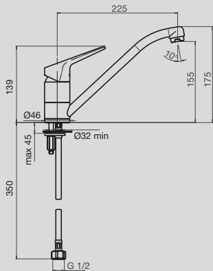
Solus MK2 Standard Sink Mixer
