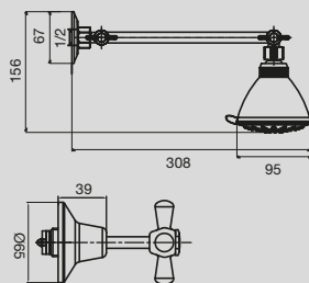
Bristol Deluxe Shower Set
