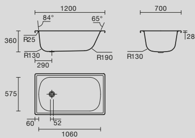
Bristol 1200mm x 700mm x 360mm Enamelled Pressed Steel Inset Bath
