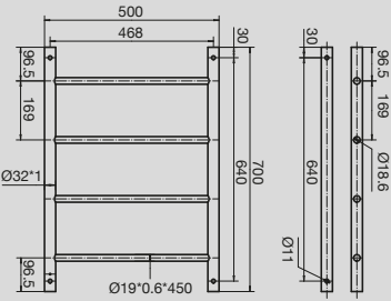
Solus MK2 Heated Towel Rail 700mm h x 500mm w
