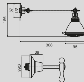
Bristol Deluxe Shower Set Lever Handle
