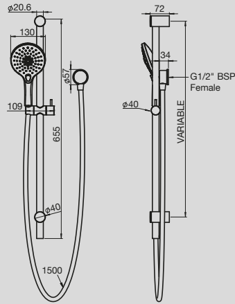
Domaine 3 Function Brass Rail Shower
