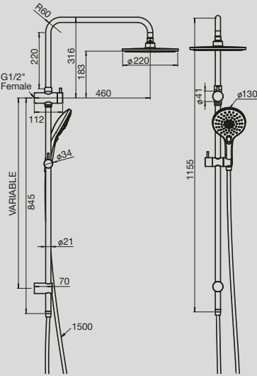
Domaine Twin Rail Shower
