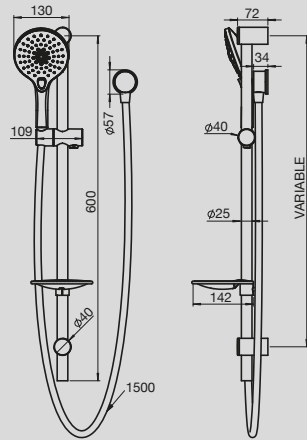
Domaine 3 Function Rail Shower
