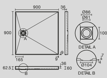
Solus 900 x 900mm Tile Over Shower Tray with Rear Waste Base Only
