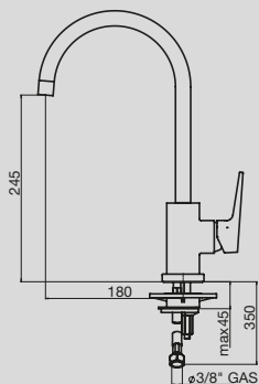
Solus MK2 Gooseneck Sink Mixer
