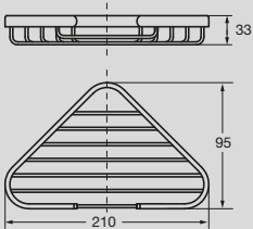
Solus Corner Wire Basket
