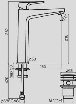
Solus MK2 Extended Basin Mixer
