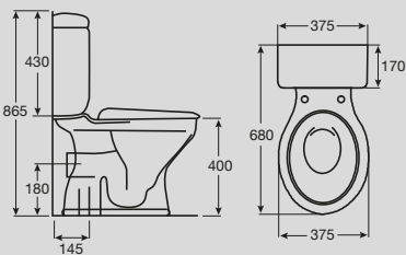
Solus Round Close Coupled S Trap Toilet Suite
