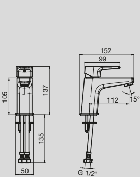
Solus MK3 Basin Mixer
