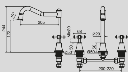
Canterbury English Hob Spa Set
