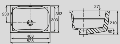
Solus Under Counter Basin 530 x 365mm
