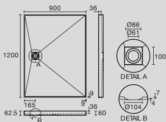
Solus 1200 x 900mm Tile Over Shower Tray with Rear Waste Base Only
