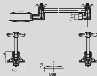
Bristol Shower Set
