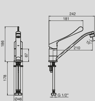
Solus MK3 Extended Lever Standard Sink Mixer
