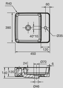
Domaine Counter Basin
