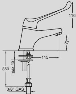
Solus MK2 Basin Mixer with Extended Lever Handle
