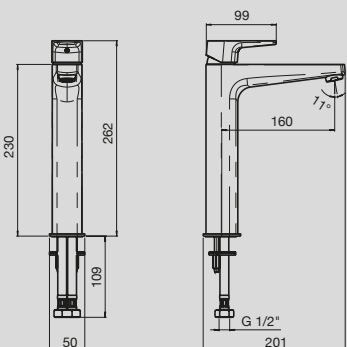
Solus MK3 Extended Basin Mixer
