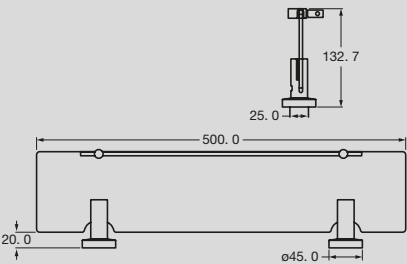
Solus MK2 Glass Shelf
