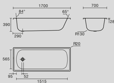
Bristol 1700mm x 700mm x 390mm Enamelled Pressed Steel Inset Bath
