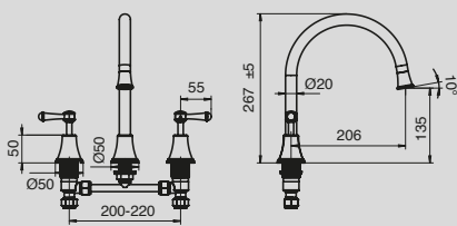
Canterbury Hob Spa Set Lever
