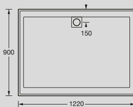
Solus 1200 x 900mm Shower Base
