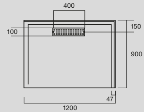
Domaine MK2 900 x 1200mm Shower Base
