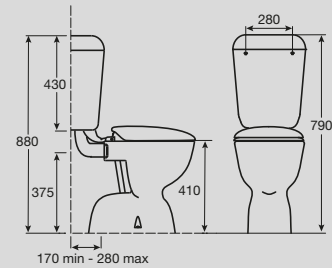
Solus Round Link Toilet Suite
