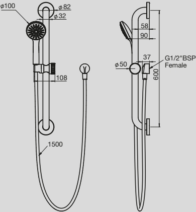
Solus MK2 1 Function 600mm Grab Rail Shower
