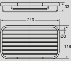
Solus Large Rectangular Wire Basket
