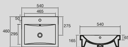
Solus Semi Inset Basin 540 x 460mm
