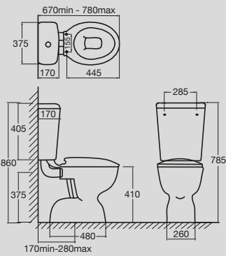
Solus Square Link Toilet Suite
