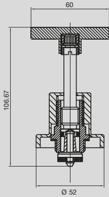
Solus Basin Top Assemblies
