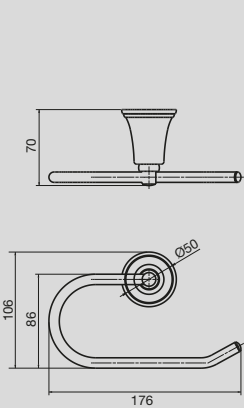
Canterbury Toilet Roll Holder
