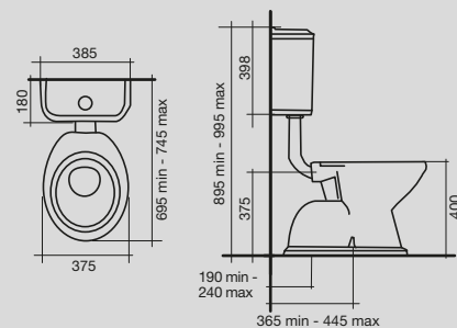
Canterbury Low Level Toilet Suite
