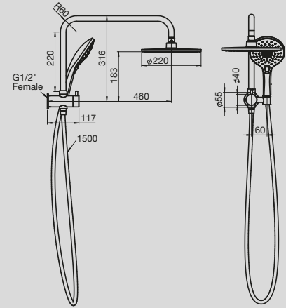
Domaine Short Twin Rail Shower
