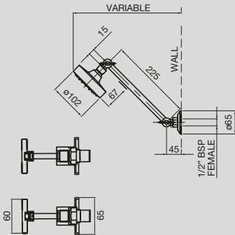
Solus Shower Set
