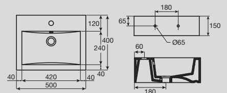
Solus Wall Basin 500 x 400mm
