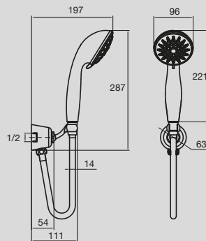
Bristol Hand Shower with Wall Bracket
