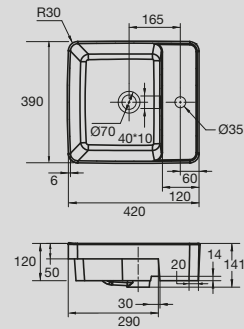
Domaine Semi Recessed Basin
