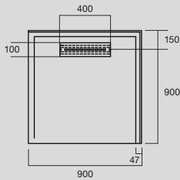
Domaine MK2 900 x 1200mm Shower Base
