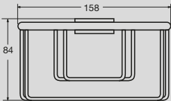
Solus Shower Rail Basket
