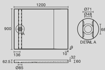
Solus 900 x 1200mm Tile Over Shower Tray with Rear Channel Base Only
