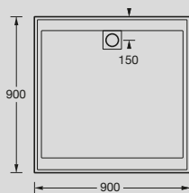
Solus 900 x 900mm Shower Base
