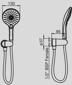
Domaine 3 Function Hand Shower
