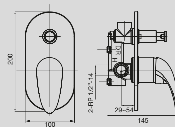
Bristol MK2 Shower Mixer Diverter
