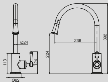
Canterbury Pull Out Sink Mixer
