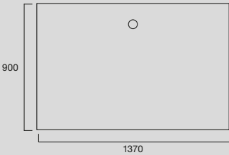
Bristol MK2 Torbex MK2 1370 x 900mm Rectangle Shower Base
