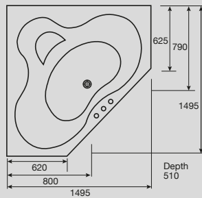
Solus MK2 Corner Santai Spa
