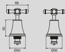
Canterbury Wall Top Assemblies
