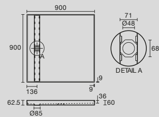
Solus 900 x 900mm Tile Over Shower Tray with Rear Channel Base Only
