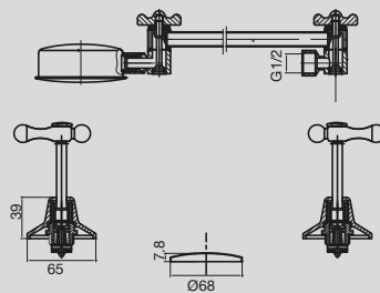
Bristol Shower Set Lever Handle
