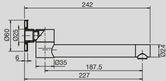
Solus MK2 Swivel Bath Outlet
