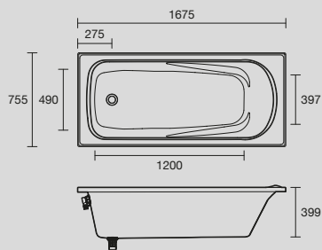
Solus 1675 MK2 Rectangular Inset Bath
