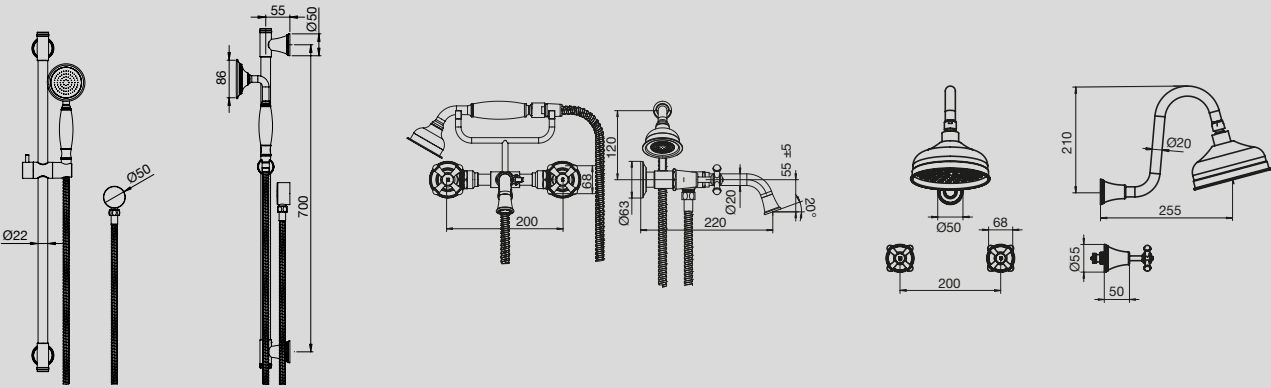
Canterbury Rail Shower
