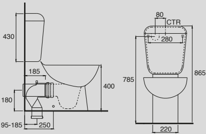
Solus Round Close Coupled Back to Wall Toilet Suite
