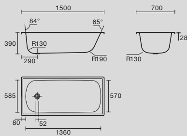
Bristol 1500mm x 700mm x 390mm Enamelled Pressed Steel Inset Bath
