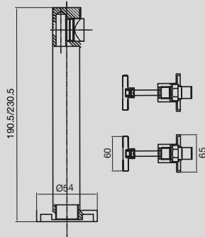
Solus Bath Set
