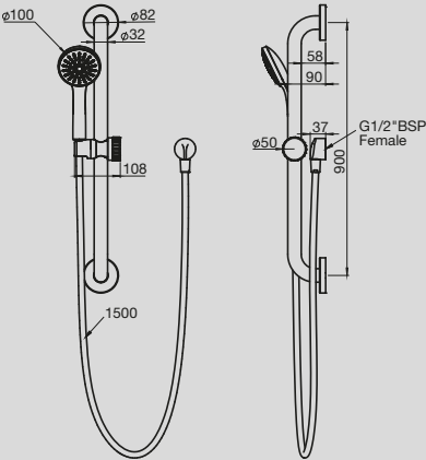
Solus MK2 1 Function 900mm Grab Rail Shower
