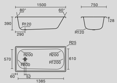
Bristol 1500mm x 750mm x 390mm Enamelled Pressed Steel Inset Bath
