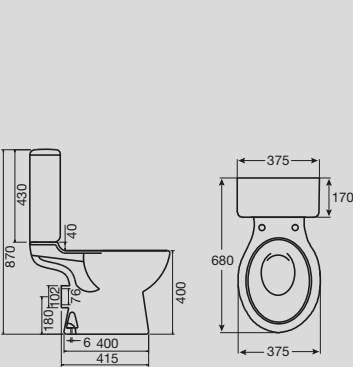
Solus Round Close Coupled P Trap Toilet Suite
