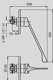
Bristol MK2 Shower Mixer with Extended Lever Handle
