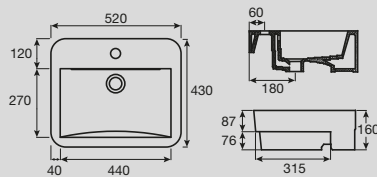
Solus Semi Recessed Basin 520 x 430mm
