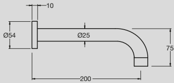
Solus Curved Bath Outlet
