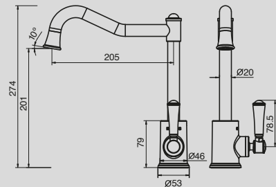
Canterbury English Sink Mixer
