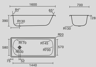
Bristol 1600mm x 700mm x 390mm Enamelled Pressed Steel Inset Bath
