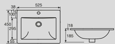
Solus Vanity Basin 525 x 450mm
