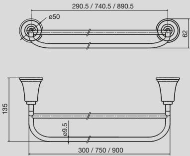
Canterbury Double Towel Rail 300mm / 750mm / 900mm
