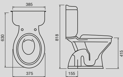
Canterbury Close Coupled Toilet Suite
