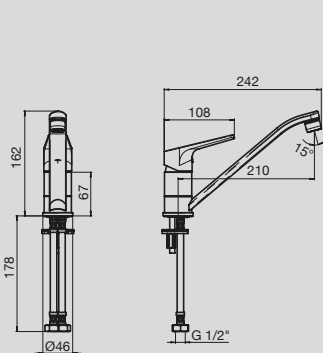
Solus MK3 Standard Sink Mixer
