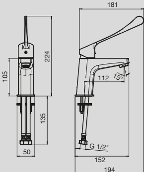
Solus MK3 Extended Lever Basin Mixer
