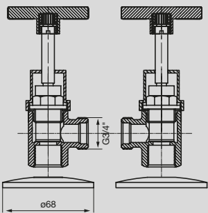
Solus Washing Machine Stops
