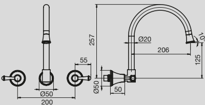
Canterbury Wall Sink Set Lever
