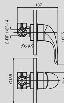
Bristol MK2 Shower Mixer
