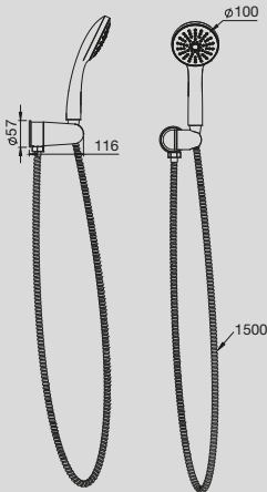
Solus MK2 1 Function Hand Shower
