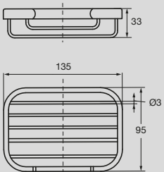
Solus Rectangular Wire Soap Basket
