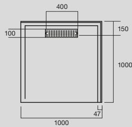
Domaine MK2 1000 x 1000mm Shower Base
