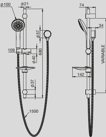
Solus MK2 3 Function Rail Shower
