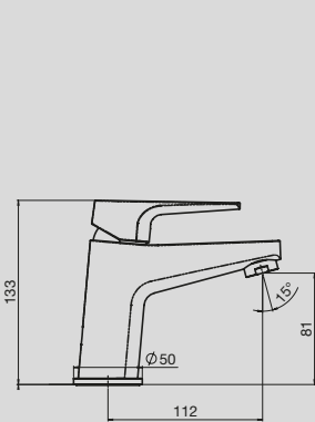
Solus MK2 Basin Mixer
