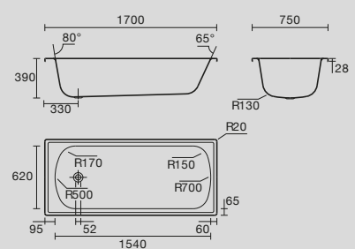
Bristol 1700mm x 750mm x 390mm Enamelled Pressed Steel Inset Bath
