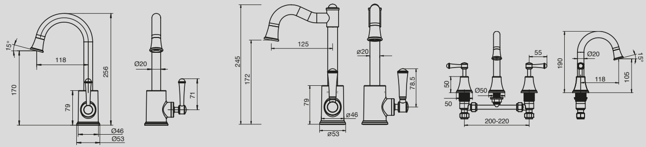
Canterbury Basin Mixer
