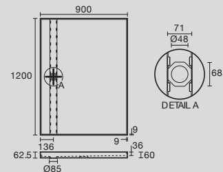
Solus 1200 x 900mm Tile Over Shower Tray with Rear Channel Base Only
