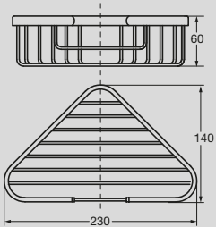
Solus Large Wire Corner Basket
