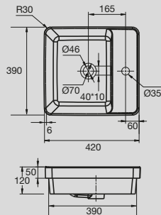
Domaine Semi Inset Basin
