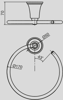
Canterbury Towel Ring
