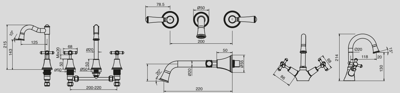
Canterbury English Basin Set
