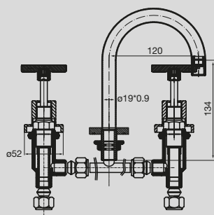
Solus Basin Set
