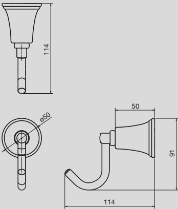
Canterbury Robe Hook
