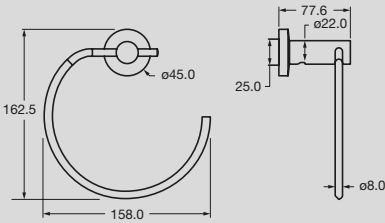
Solus MK2 Guest Towel Ring
