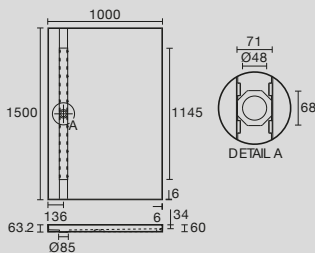
Solus 1500 x 1000mm Tile Over Shower Tray with Rear Channel Base Only
