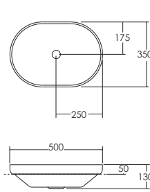
Venice 500 Oval Semi Inset
