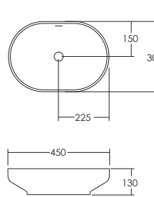
Venice 450 Oval with Overflow
