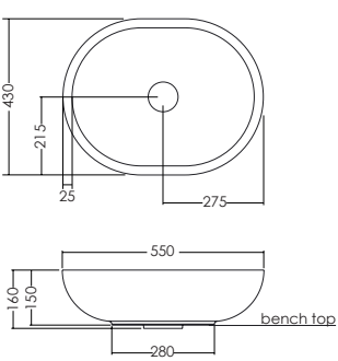
Villa 550 oval Bench mounted
