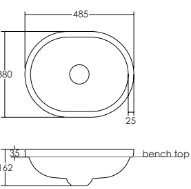
Villa 485 oval Semi inset
