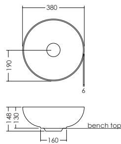
Villa 380 round - thin edge Bench mounted
