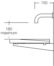
Outlet detail for 800 Washplane®
