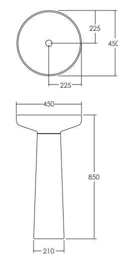
Venice 450 Round Pedestal
