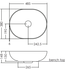
Villa 485 oval - thin edge Bench mounted
