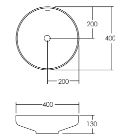
Venice 400 Round with Overflow
