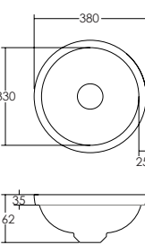
Villa 380 round Semi inset
