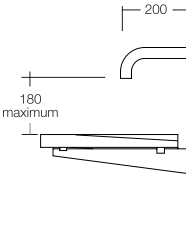
Outlet detail for 1200/1600/2100 Washplane®
