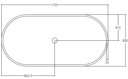
Villa 1725 freestanding bath
