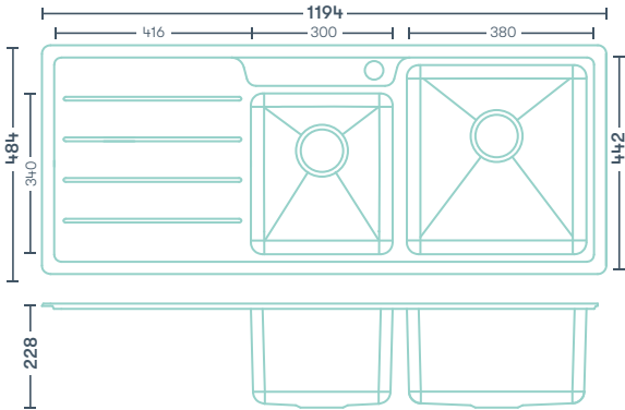
1 3/4 Drainer RHB 1 Taphole 1194mm x 484mm 2403006
