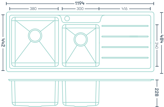
1 3/4 Drainer LHB 1 Taphole 1194mm x 484mm 2403005
