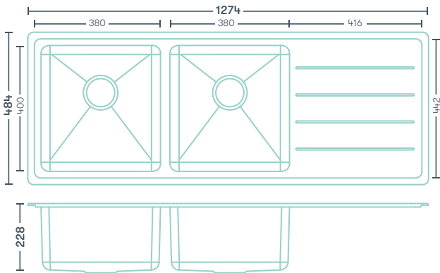
Double Drainer LHB No Taphole 1274mm x 484mm 2403003
