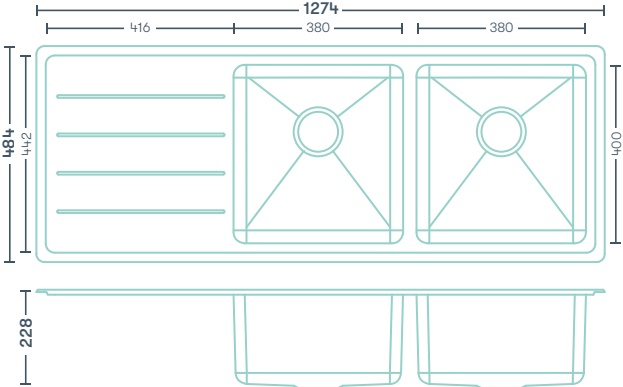
Double Drainer RHB No Taphole 1274mm x 484mm 2403004
