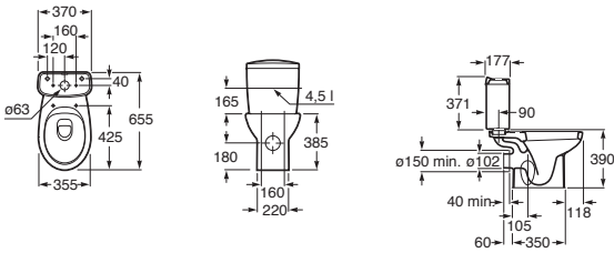
Victoria Close Coupled Toilet Suite - P Trap
