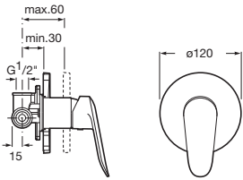
Logica-N Shower Mixer
