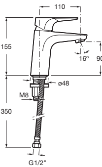
Atlas Basin Mixer
