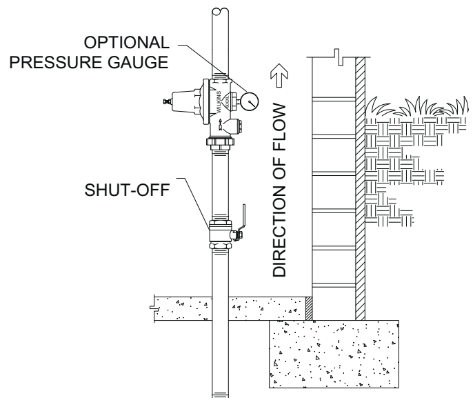
VERTICAL INSTALLATION
