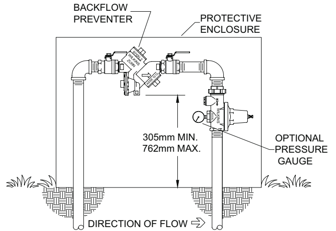
OUTDOOR INSTALLATION
