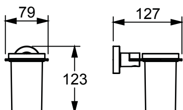
Tumbler Holder
