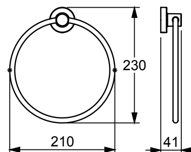
Towel Ring
