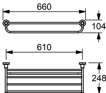
Towel Rack
