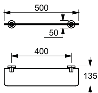
Shelf (Glass)
