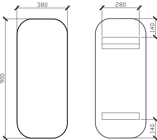
380W x 42D X 900H
