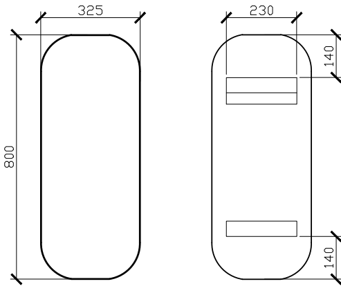
325W x 42D X 800H
