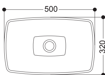
H10 Rectangle Above Counter Basin 500 x 320mm
