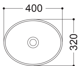
H10 Oval Above Counter Basin 400 x 320mm
