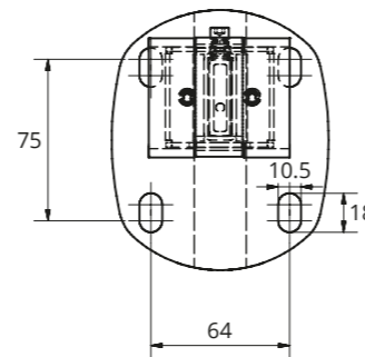
Dimensions of base-plate for Floor Bracket SK
