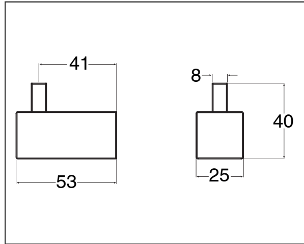
Robe Hook 9508785
