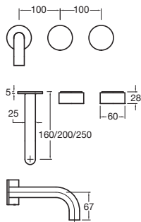
Pure Wall Basin Hostess System
