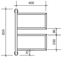
Mood Edit Heated Towel Rail Swivel 400x635mm
