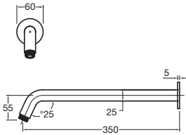
Mood Edit Horizontal Shower Arm 350mm
