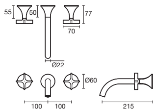
Oria Wall Basin Set Cross
