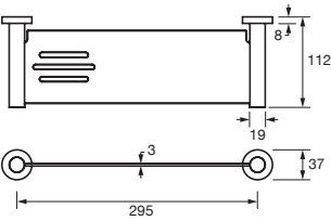
Mood Edit Shower Shelf
