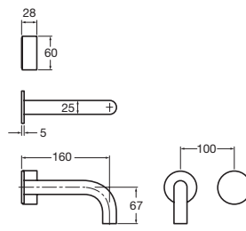
Pure Progressive Wall Basin Mixer System
