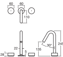
Pure Basin Set
