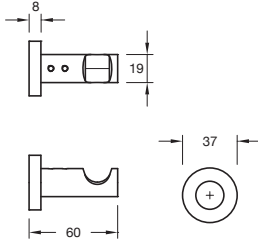
Mood Edit Robe Hook
