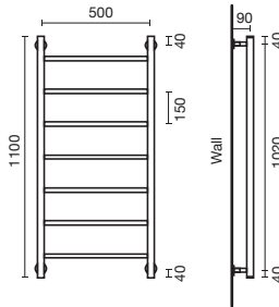
Mood Edit Heated Towel Rail 500x1100mm
