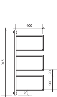
Mood Edit Heated Towel Rail Swivel 400x945mm
