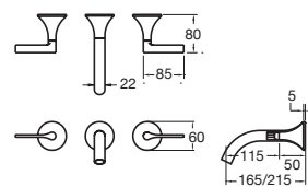
Oria Wall Basin Set Lever
