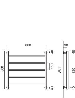
Mood Edit 800x800mm Heated Towel Rail
