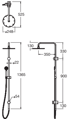
Mood Edit Twin Square Waterrail Shower
