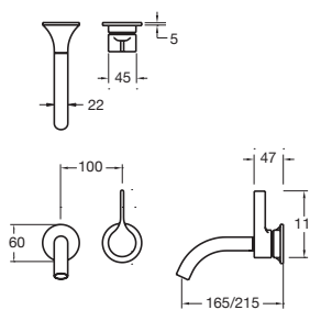
Oria Wall Bath Mixer Set
