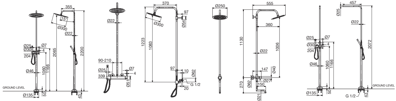
Inox Freestanding Twin Rail Shower with Overhead Shower
