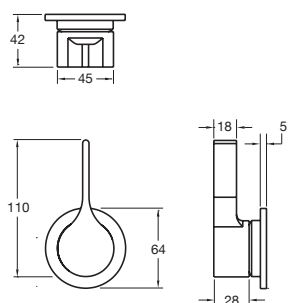
Oria Shower/Bath Mixer
