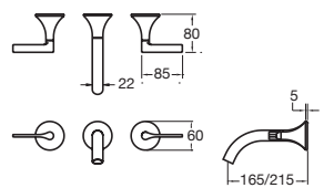
Oria Wall Bath Set Lever
