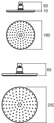
Mood Edit Shower Head
