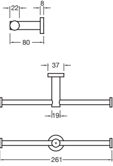
Mood Edit Double Toilet Roll Holder
