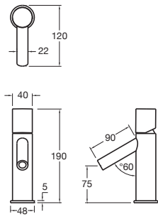
Pure Basin Mixer
