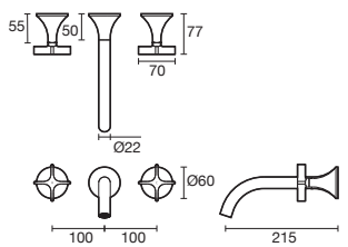
Oria Wall Bath Set Cross
