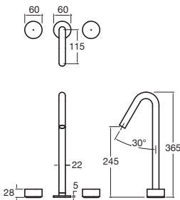
Pure Vessel Basin Set
