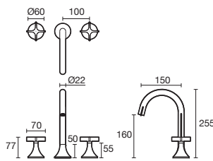
Oria Basin Set Cross
