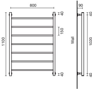
Mood Edit Heated Towel Rail 800x1100mm
