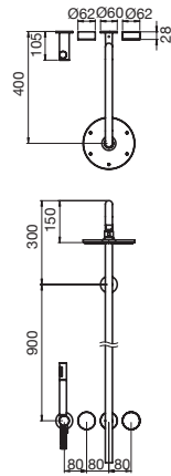
Mood Edit Column Shower Mixer System with Hand Shower
