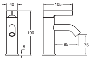
Oria Basin Mixer
