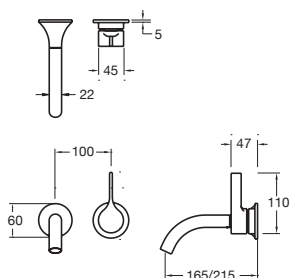
Oria Wall Basin Mixer Set
