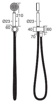
Mood Edit Round Hand Shower
