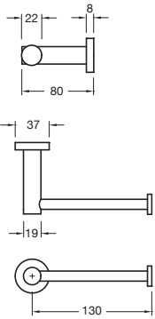
Mood Edit Toilet Roll Holder
