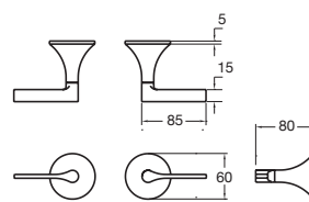
Oria Wall Top Assembly Lever
