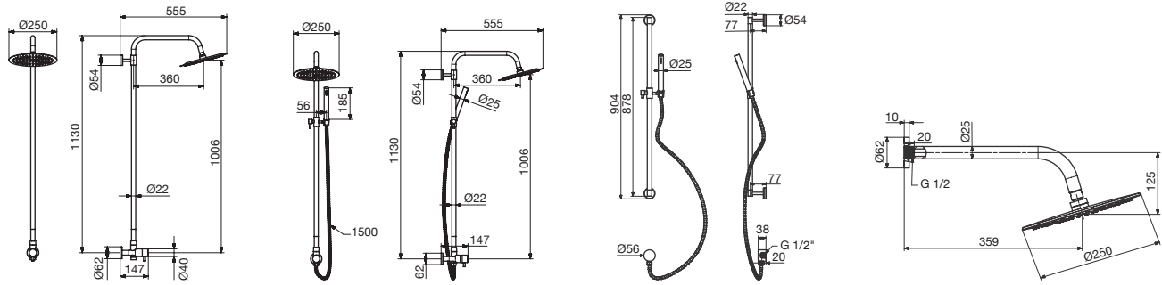
Inox Overhead Rail Shower
