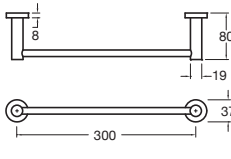
Mood Edit Guest Towel Rail
