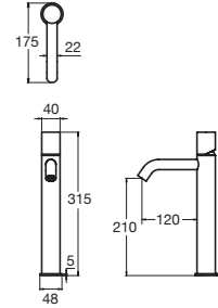
Pure Curve Extended Basin Mixer
