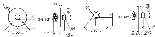
Inox Shower Mixer – Large Backplate
