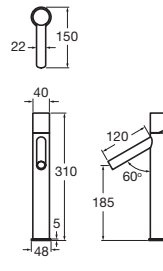
Pure Extended Basin Mixer
