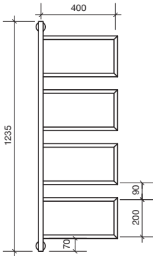
Mood Edit Heated Towel Rail Swivel 400x1235mm
