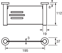
Mood Edit Soap Dish
