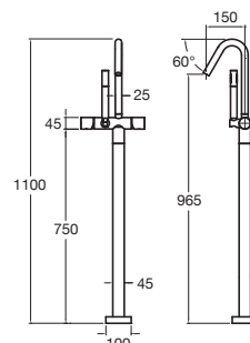
Pure Floor Mounted Mixer with Hand Shower
