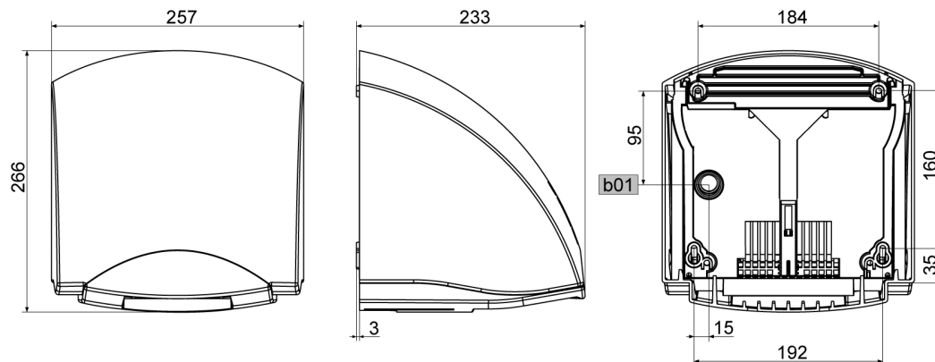
HTE 5 Dimension Drawing
