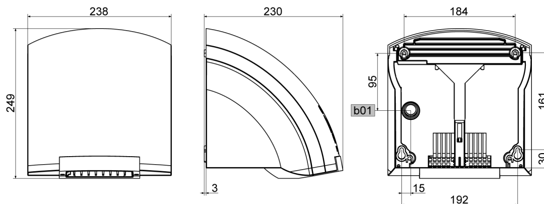
HTE 4 Dimension Drawing
