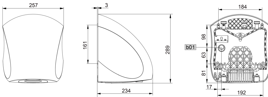
Ultronic S / W Dimension Drawing
