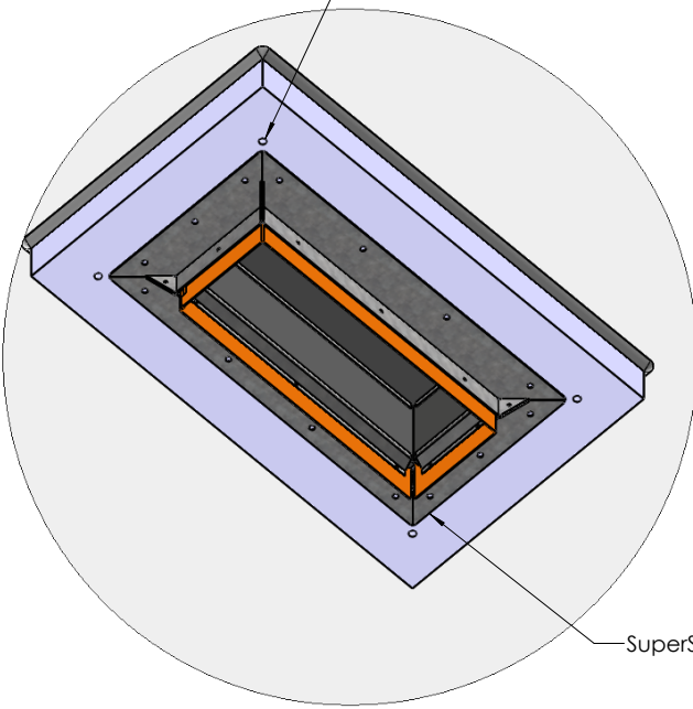
DETAIL D - Bottom Side View
