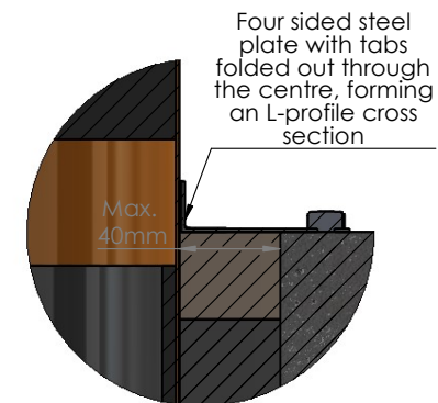
Enlarged Updated Flange Up to 40mm annular gaps*
