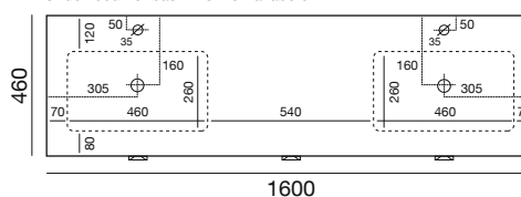
Under-counter basin - CIBO Lavabo 3
