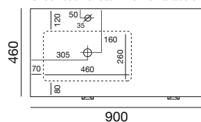
Under-counter basin - CIBO Lavabo 3
