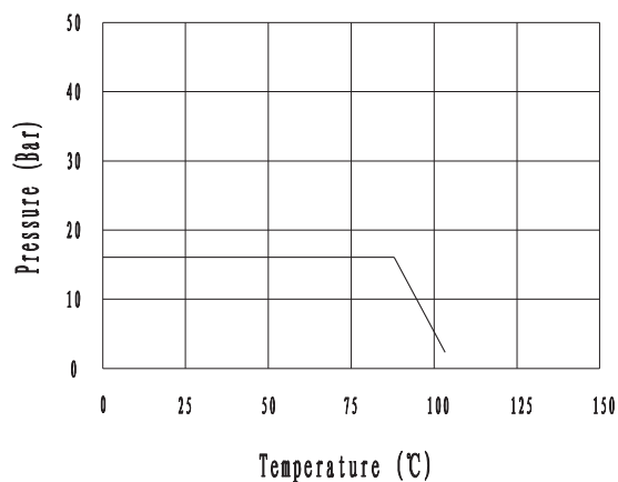
Pressure/Temperature Diagram
