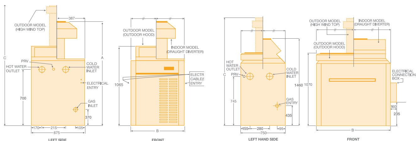
Models 200, 280, 350, 430 (Indoor/Outdoor)
