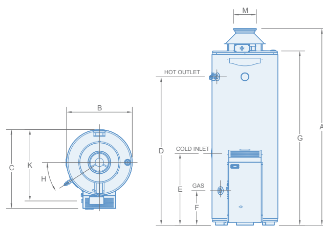
Indoor Models
