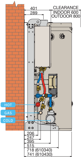
Wall Mount
