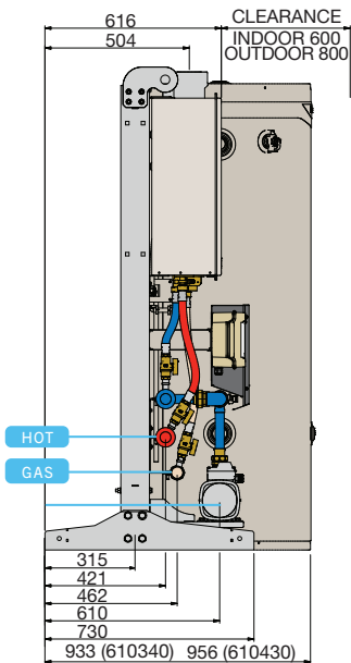
Floor Mount
