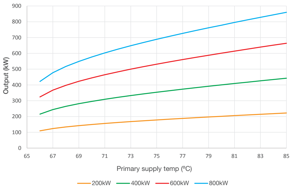
Rheem Crossflow Maximum Output ( T_{in}^{15^{\circ}\text{C}} - T_{in}^{65^{\circ}\text{C}} ) vs. Primary supply temp
