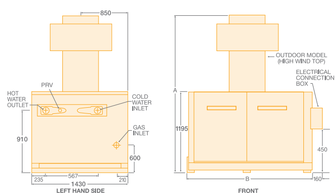
Models 2004, 2404, 2804 2 , 3304 2 , 3804 2 (Outdoor)
