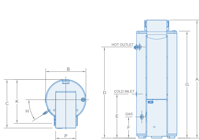
Outdoor Models
