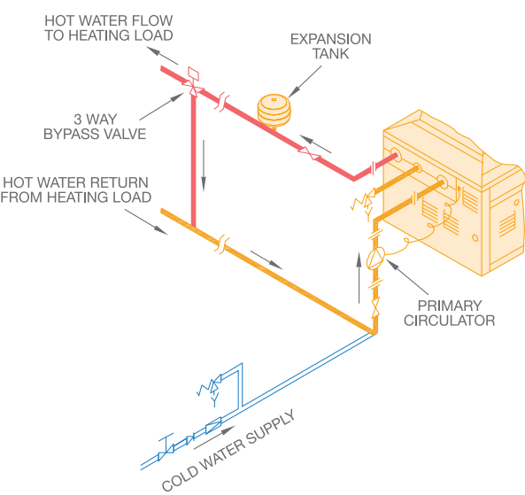
Single Mechanical Heating System
