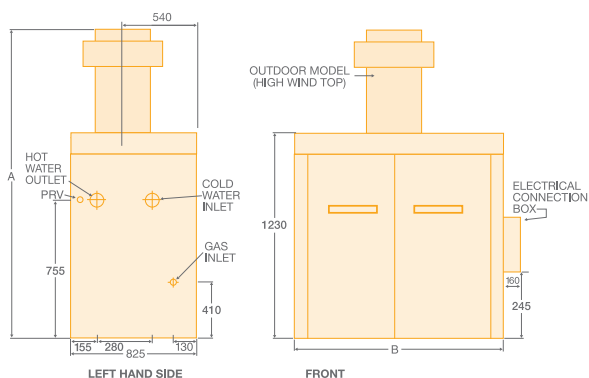
Models 972, 1142, 1242, 1362, 1662, 1852 (Outdoor)
