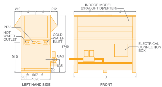
Models 2214, 2634, 3164, 3694, 4224 (Indoor)
