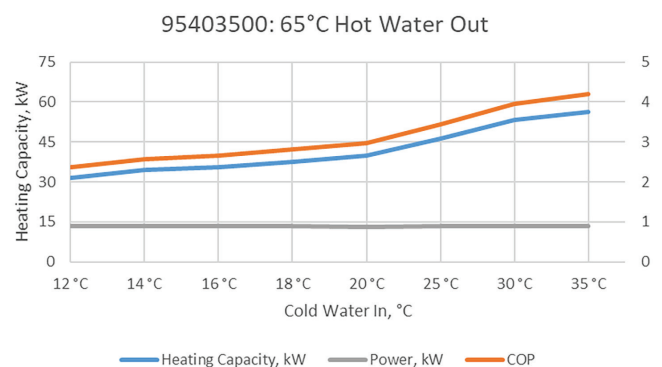
35 kW W2W COP and Heating Capacity
