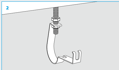
Step 2 – Slide pear clip over thread and attached second nut below clip, adjusting to required height. Do not tighten top nut, leave a gap of approximately 5mm.
