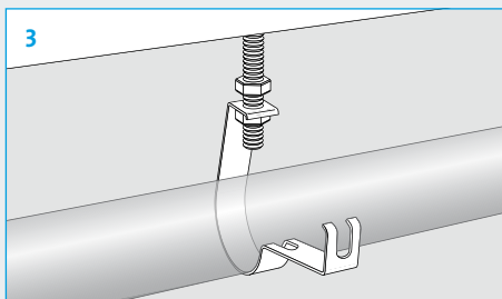
Step 3 – Hang pipe on bracket. Pear clip will hold pipe temporarily until fastened.
