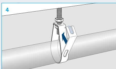
Step 4 – Simply push edge of pear clip upwards as shown. Clip will fit around bolt and snap into place locking shut.
