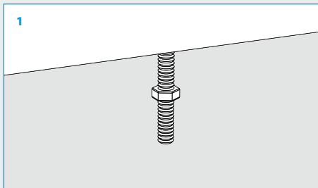
Step 1 – Trim All Thread to length and secure to anchor point. Spin on top nut.
