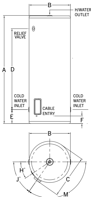
Everhot SS 250L and 315L
