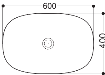
Counter Basin 600 x 400mm.
