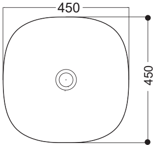
Counter Basin 450 x 450mm.
