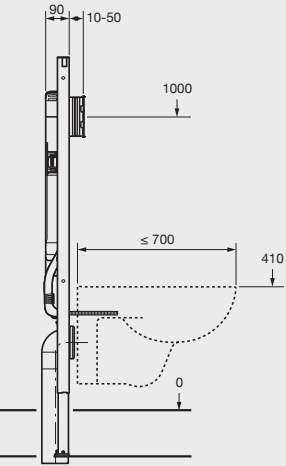
90mm Wall cavity
