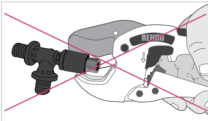
Fig. 7-24 Unapproved cutting of the PX sleeve
