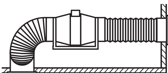
Single-Point Intake:
