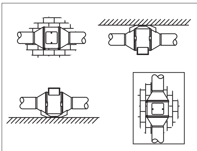
Single-Point Intake:
