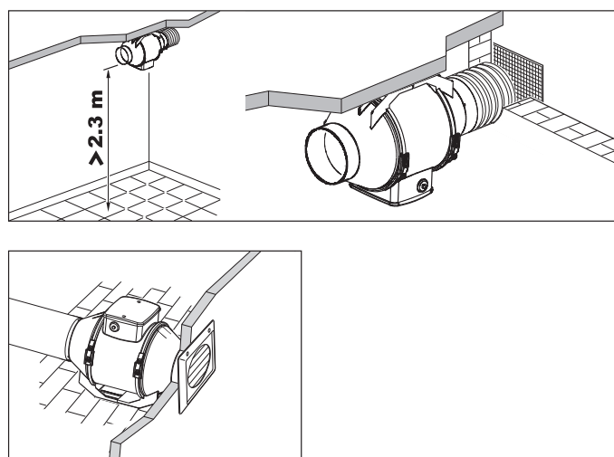
Multi-Point Intake:
