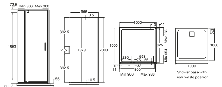
1790304 — 1000mm Rear Outlet
