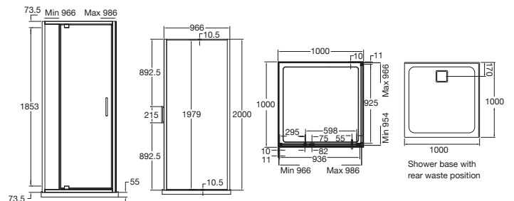
1790310 — 1000mm Rear Outlet
