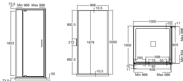
1790303 — 1000mm Centre Outlet
