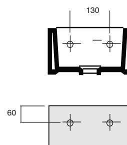
b) Rear tap hole fixing bolt detail
