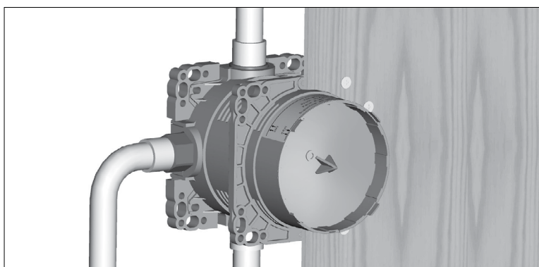
Installation behind a prefabricated wall
