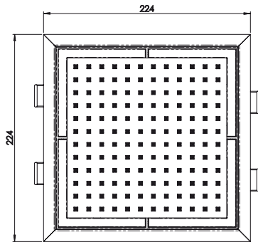
Nobili Plus Single Ceiling Shower (2 Star)
