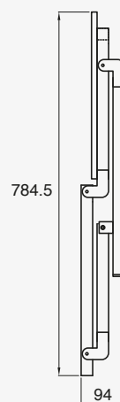
Folded view
