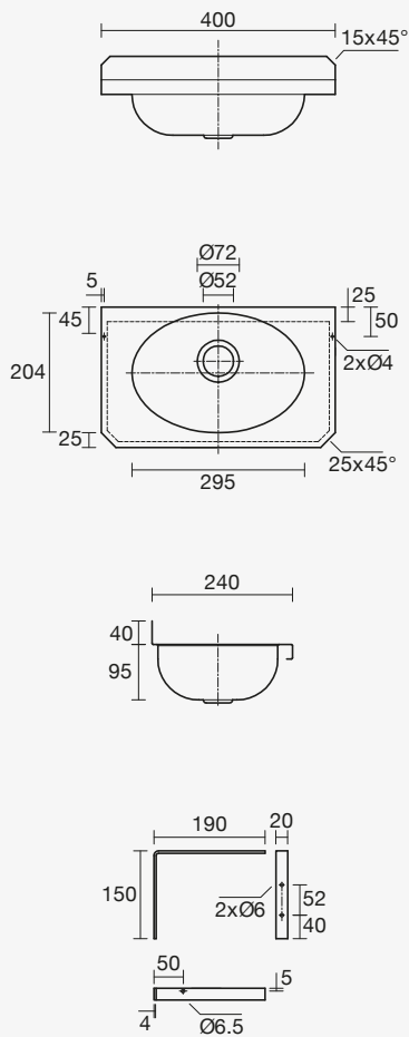
No Taphole
