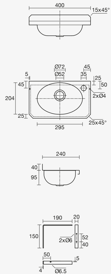
Right Taphole
