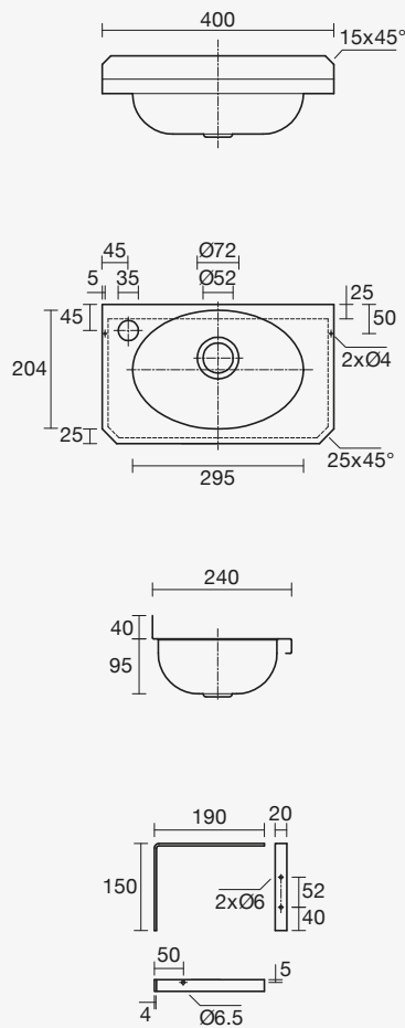
Left Taphole
