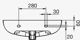
1 Taphole, 1 Overflow
